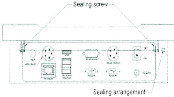
BACK VIEW
